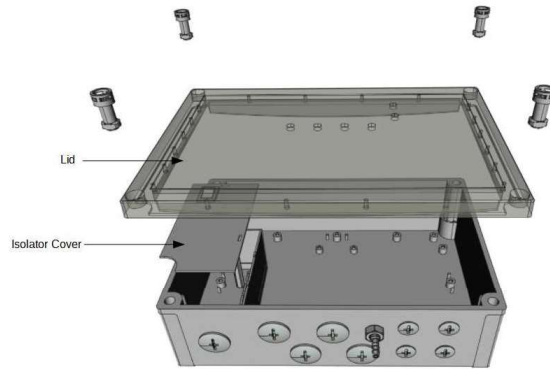
Figure 1 1002510 Lid & Cover
