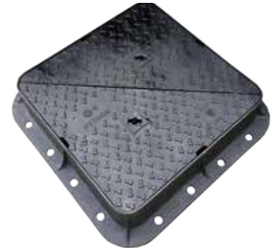
PYTHON 150
