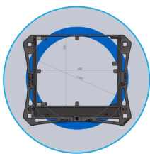
Designed To Suit A Ø450mm Gully Pot
