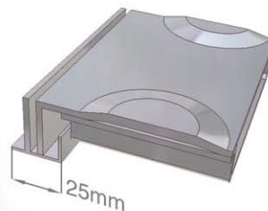
Single Seal Frame Detail
