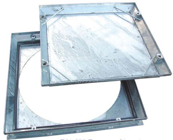
R2T-450 Recessed tray type
