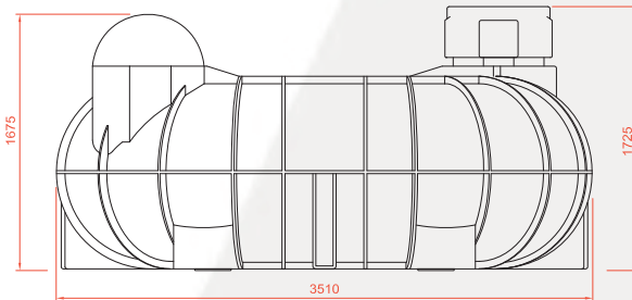
SIDE ELEVATION
