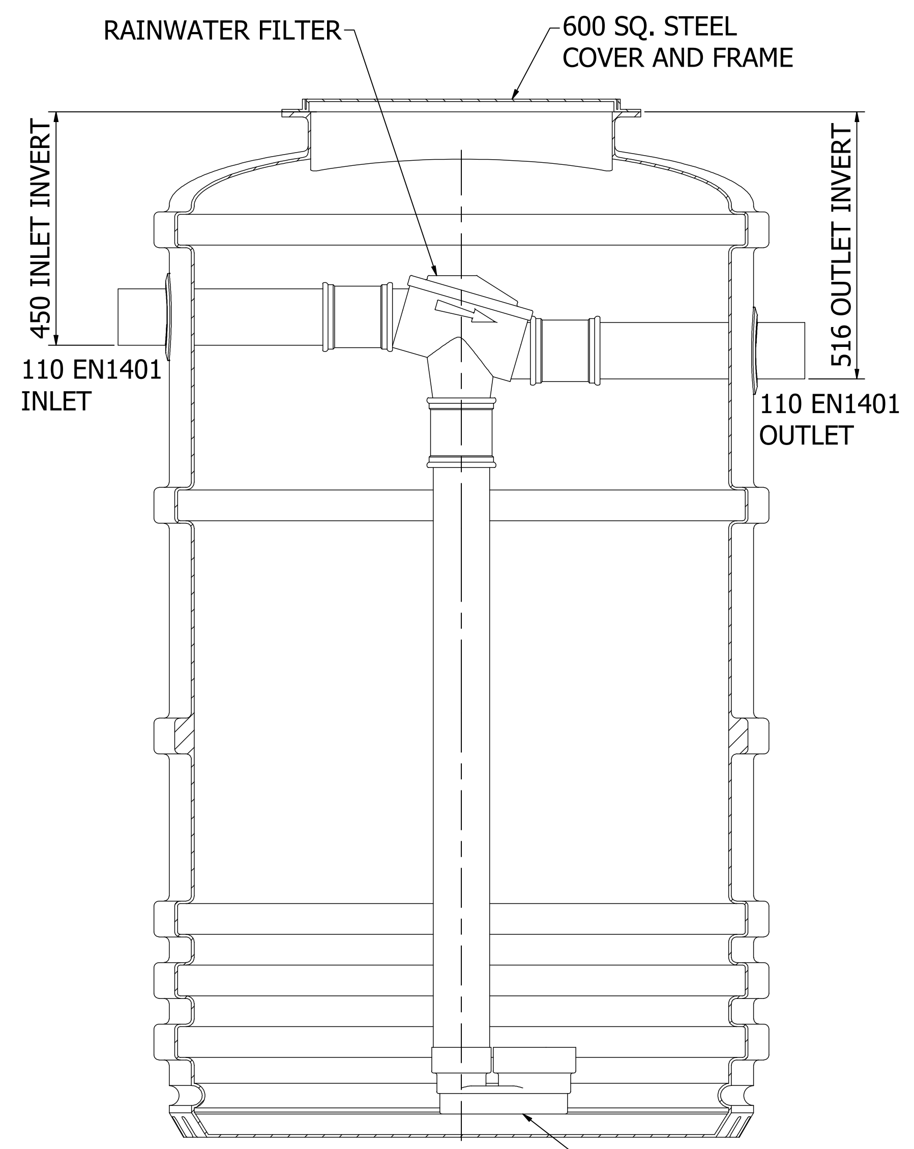
SECTION A-A SCALE 1:7.5 FLOW CALMER
