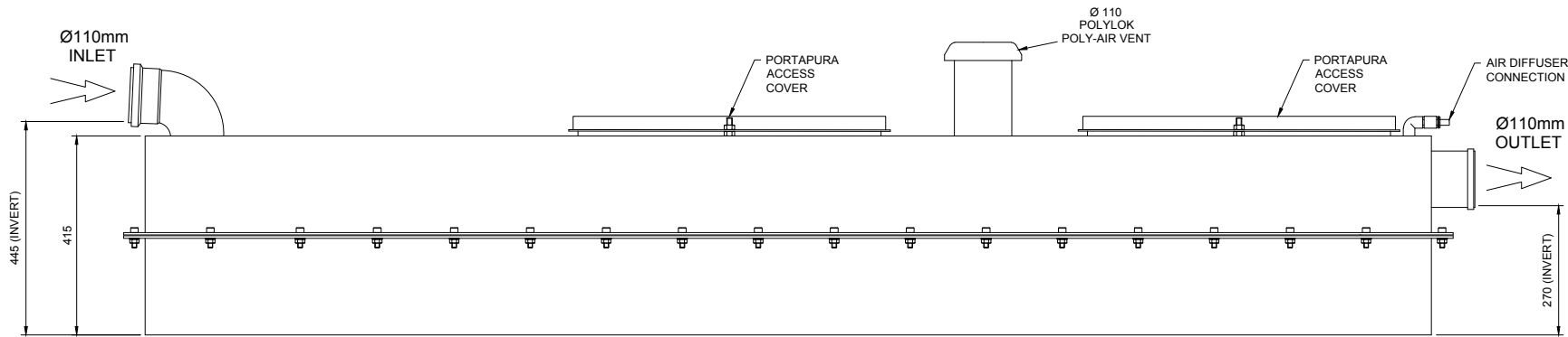
SIDE VIEW
